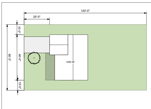
Setbacks on a typical lot.
